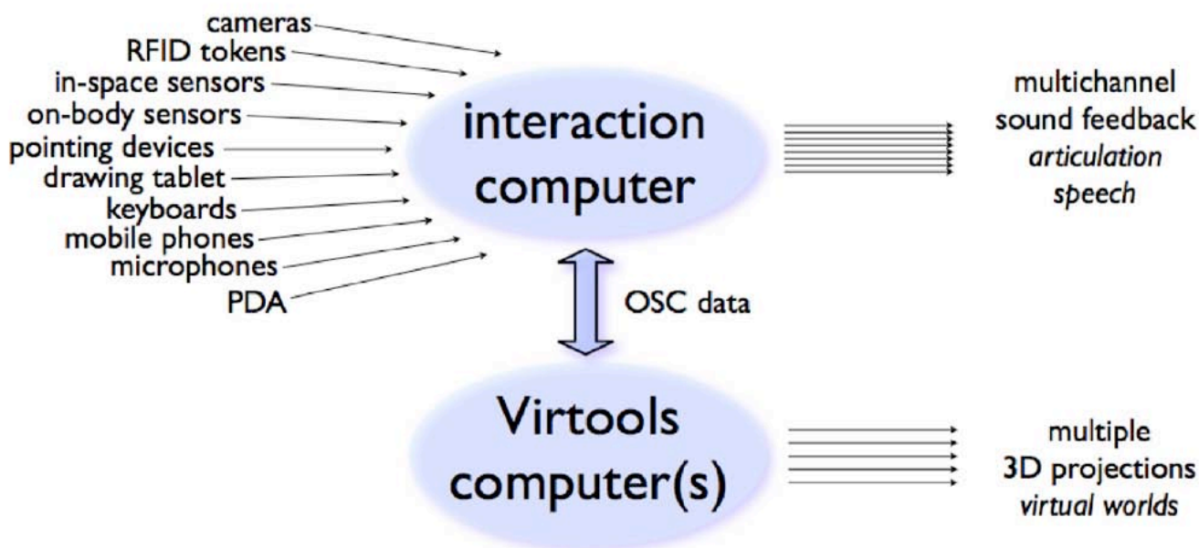
Fig. 2 Overview of the Protospace interaction system
