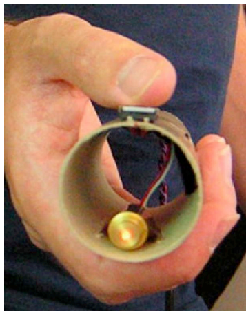
Fig. 8 The LaserTouch Pointer prototype
